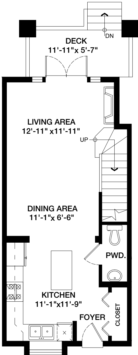
Main Floor Plan Floor Area: 490 sq.ft.
