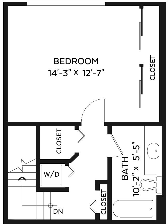
Upper Floor Plan Floor Area: 424 sq.ft.
